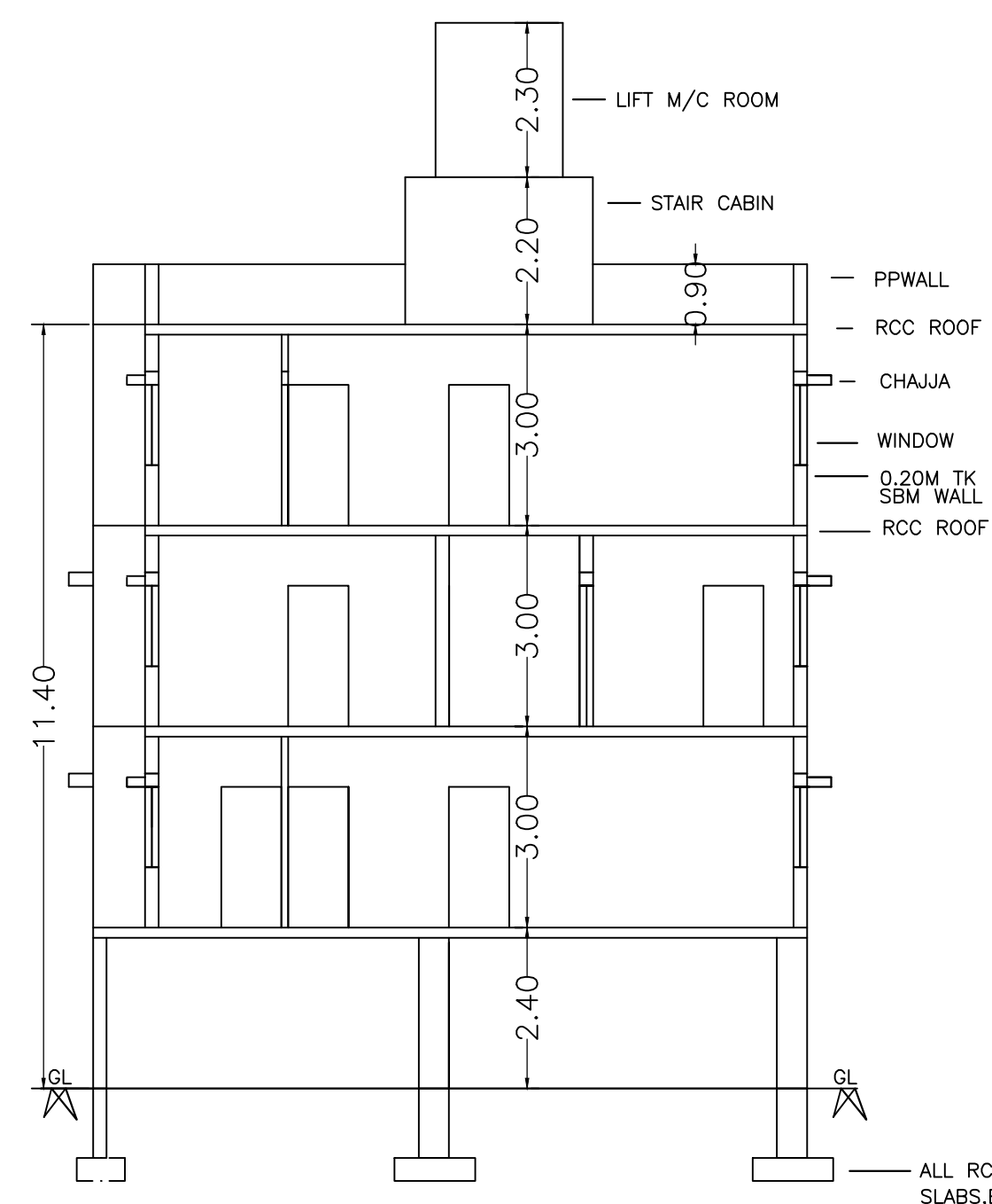
SECTION AA
